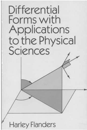
Figure 4.1. Two introductory books on the theory of differential forms.
