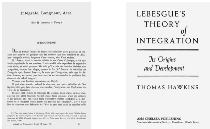
Figure 6.1. The first page of the doctorate thesis of Henri Lebesgue (1875–1941) that appeared in 1902, and an essay on the hystorical developments of Lebesgue’s integral.
