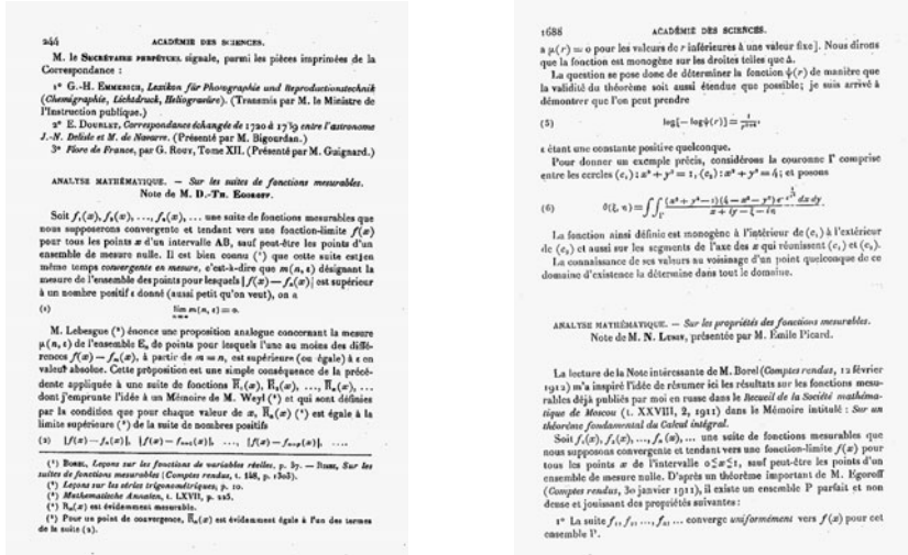
Figure 5.4. The beginning of two papers by Dimitri Egorov (1869–1931) and Nikolai Lusin (1883–1950) in which Egorov and Lusin theorems are proved.
